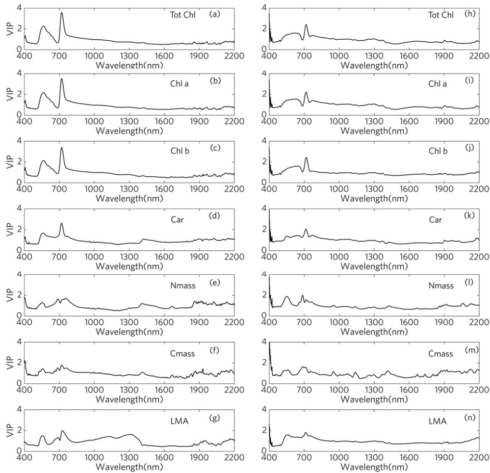
Fig. 6. Relative importance of each wavelength in variable importance on projection (VIP). VIP values from PLSR ref and PLSR tra are on the right and left, respectively.
