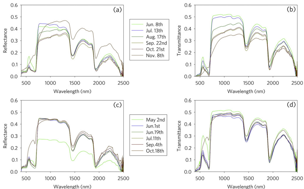
Fig. 4. Examples of leaf directional-hemispherical reflectance and transmittance measured on (a, b) Martha's Vineyard and in (c, d) Harvard Forest.
