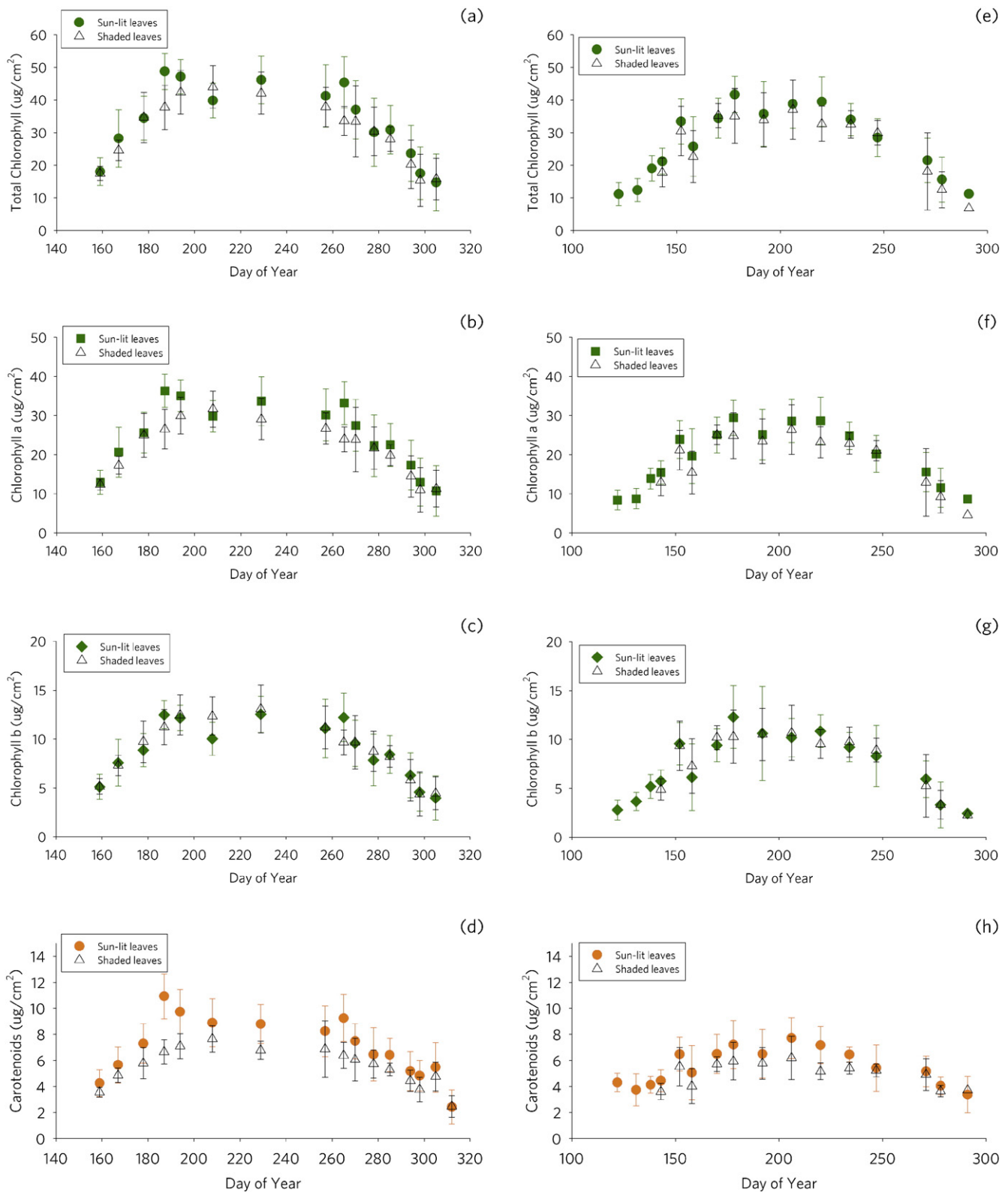
Fig. 1. Seasonal patterns of pigments of sunlit (filled) and shaded (open) leaves from two deciduous forests. Martha's Vineyard, year 2011: (a) Total chlorophyll; (b) chlorophyll a ; (c) chlorophyll b ; (d) carotenoids. Harvard Forest year 2012: (e) Total chlorophyll; (f) chlorophyll a ; (g) chlorophyll b ; (h) carotenoids. Each dot is the mean value of all the samples collected that day. Error bars are standard deviations.
