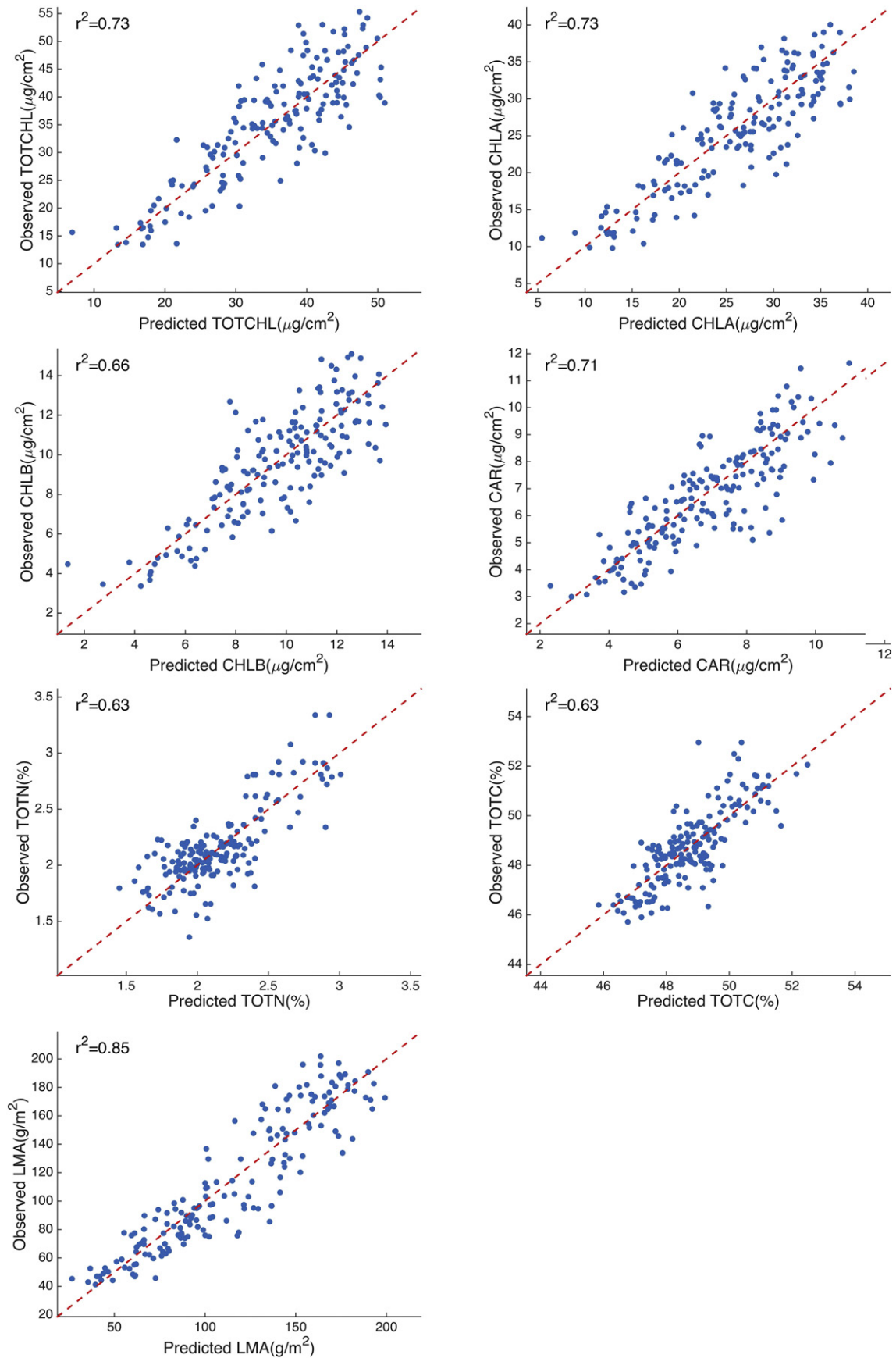
Fig. 5. Comparisons between the observed leaf traits and predicted traits from PLSR ref . For detailed statistics, refer to Tables 2 and 3. Observations are from the independent validation dataset selected using the Kennard-Stone method. The red dashed lines are 1:1 line.
