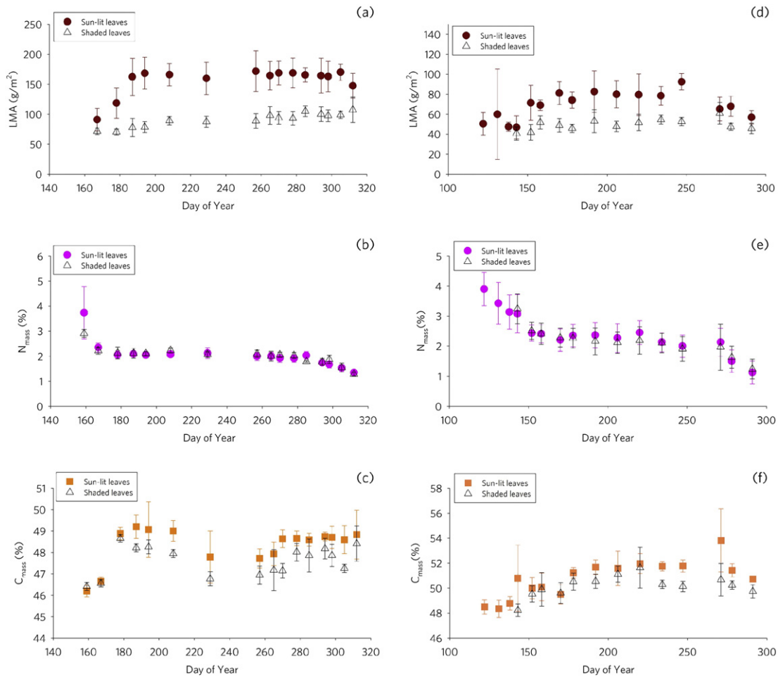
Fig. 2. Seasonal patterns of biochemical and biophysical properties of sunlit (filled symbols) and shaded (open symbols) leaves from two deciduous forest sites. Martha's Vineyard, year 2011: (a) Leaf mass per area (LMA); (b) mass-based nitrogen concentration ( N_{mass} ); (c) mass-based carbon concentration ( C_{mass} ). Harvard Forest, year 2012: (d) LMA; (e) N_{mass} ; (f) C_{mass} . Each dot is the mean value of all the samples collected that day. Error bars are standard deviations.
