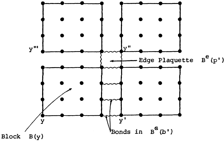
Fig. 1. Block variables for gauge fields, drawn in d=2 . Four blocks are illustrated. Let B(y) denote a block with L=4 . The L -lattice bonds illustrated are b' = yy', y'y'', y''y''', and y'''y' . These four L -bonds bound a plaquette p' . The corresponding edge plaquette B^e(p') is indicated. The bond b' has associated surface bonds B^s(b') which connect B(y) and B(y') . A few bonds connecting distinct blocks are indicated by wavy lines
