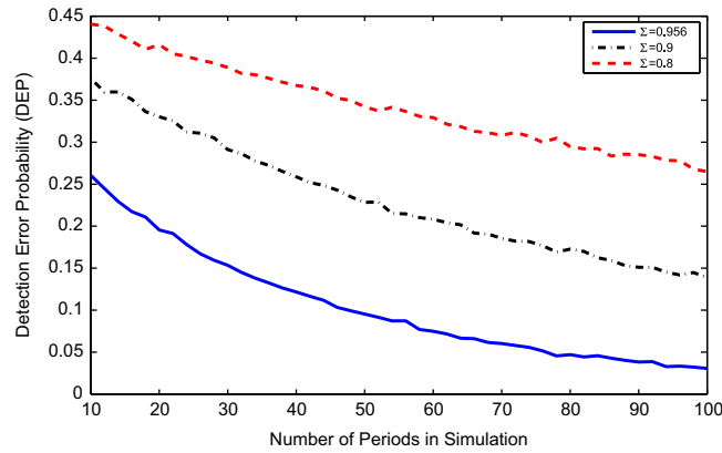
Fig. 4. Detection error probability (DEP) and the simulation length.
