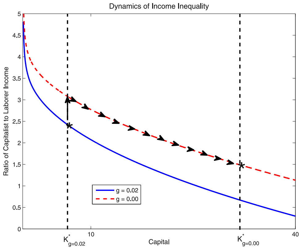
Fig. 11. Dynamics of inequality.
