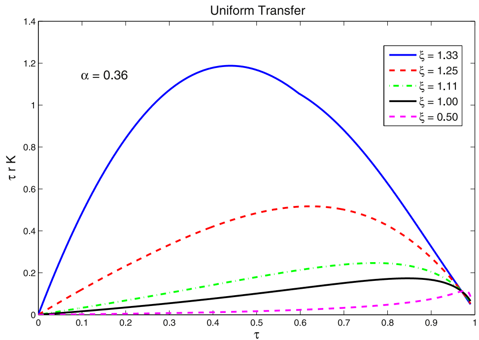
Fig. 12. Laffer curve.
