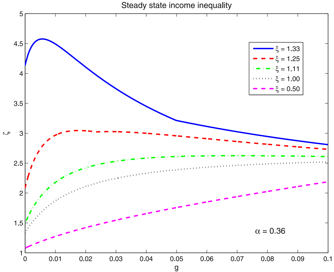
Fig. 2. Steady state inequality.
