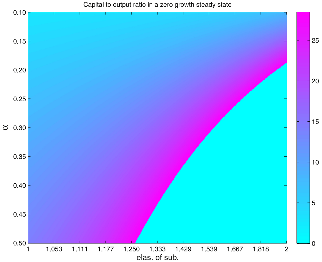
Fig. 6. Capital to income ratio in a zero growth steady state.
