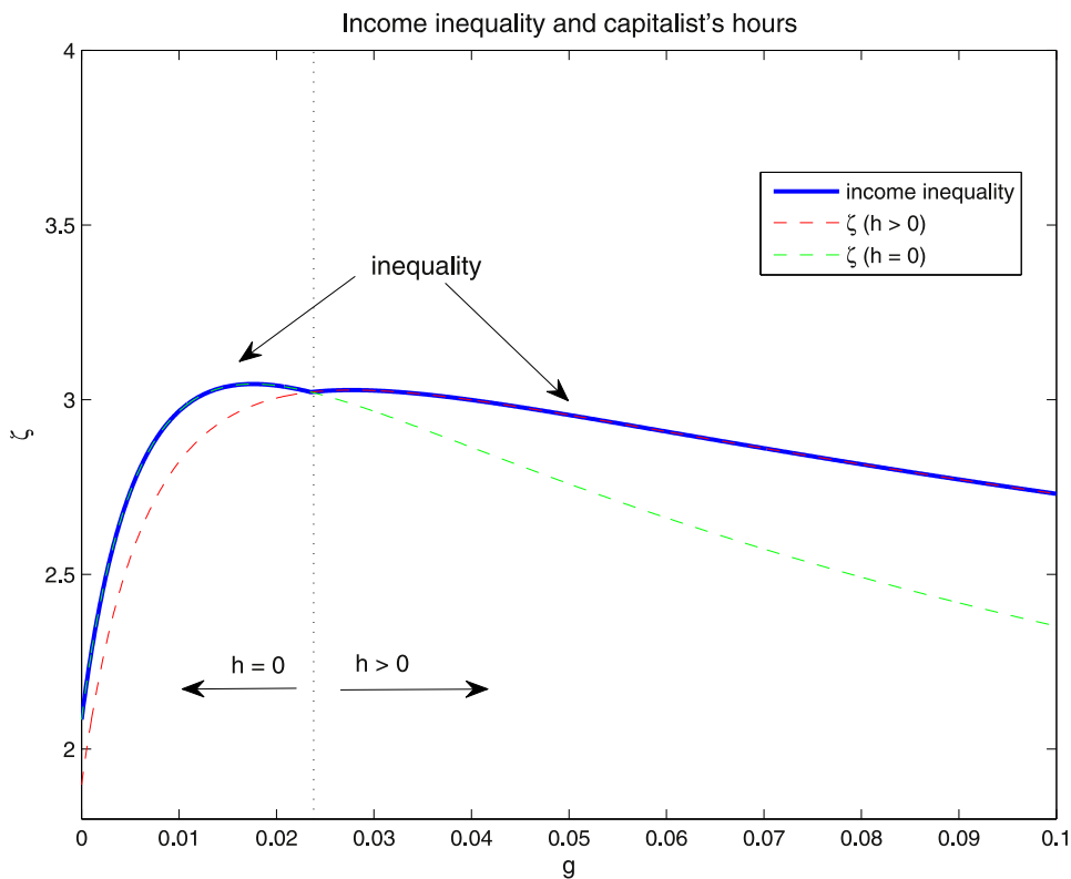
Fig. 10. Steady state inequality.
