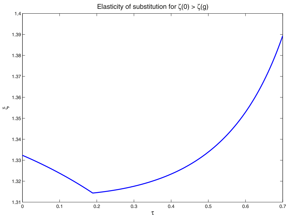
Fig. 15. Necessary elasticity of substitution to cause higher inequality with zero growth.
