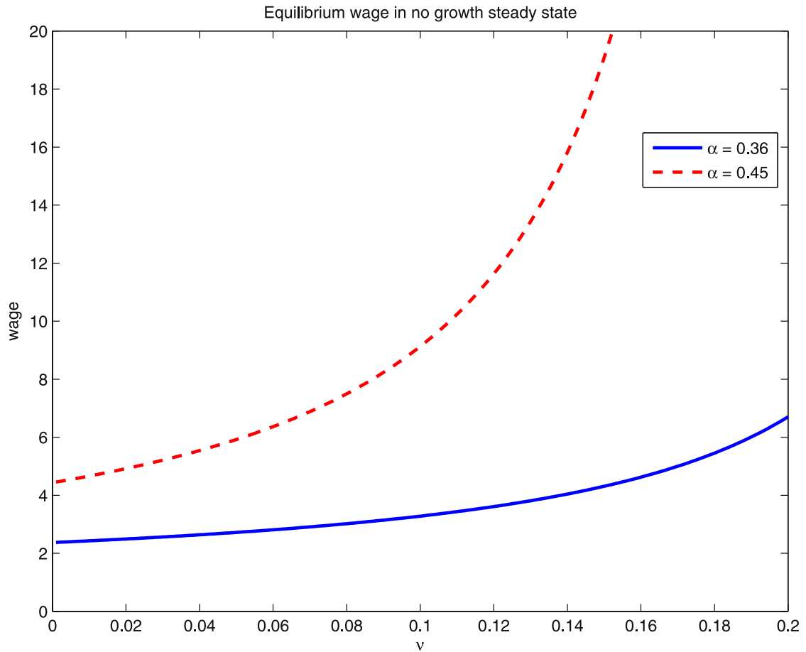
Fig. 1. Equilibrium wage in g = 0 steady state.
