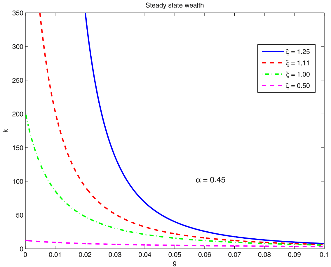
Fig. 5. Steady state wealth.
