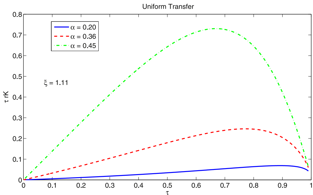
Fig. 13. Laffer curve.
