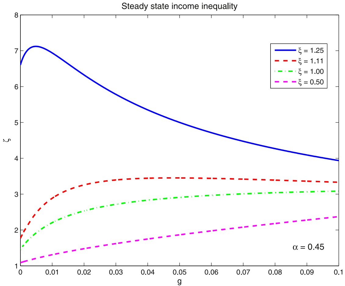
Fig. 3. Steady state inequality.
