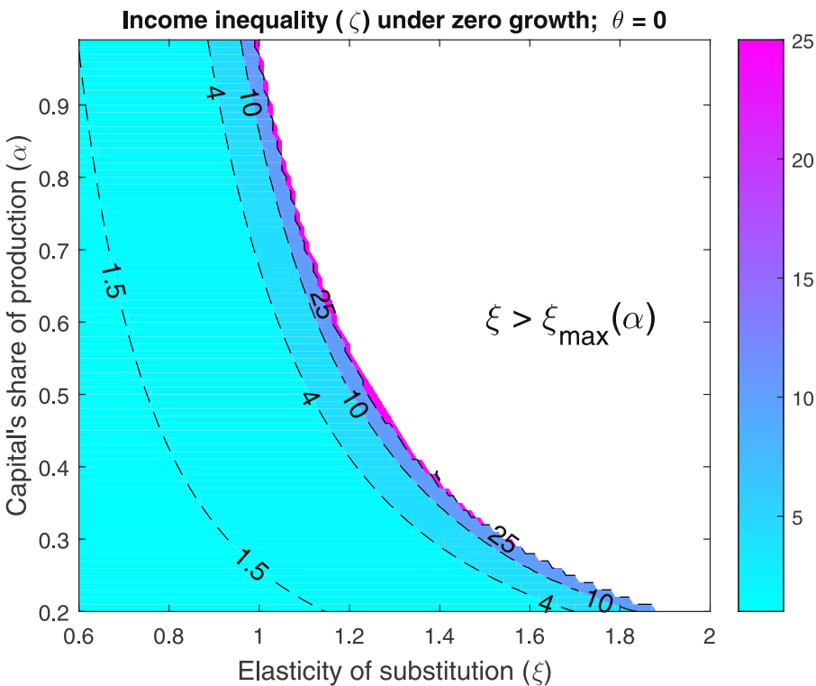
Fig. 8. Income inequality in a zero growth steady state.
