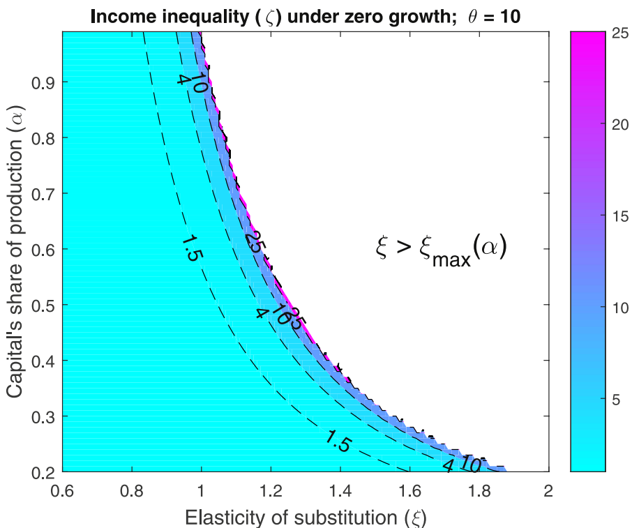
Fig. 9. Income inequality in a zero growth steady state.
