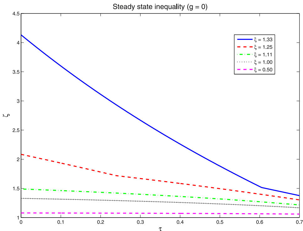
Fig. 14. Long run inequality under capital income taxation and zero growth.
