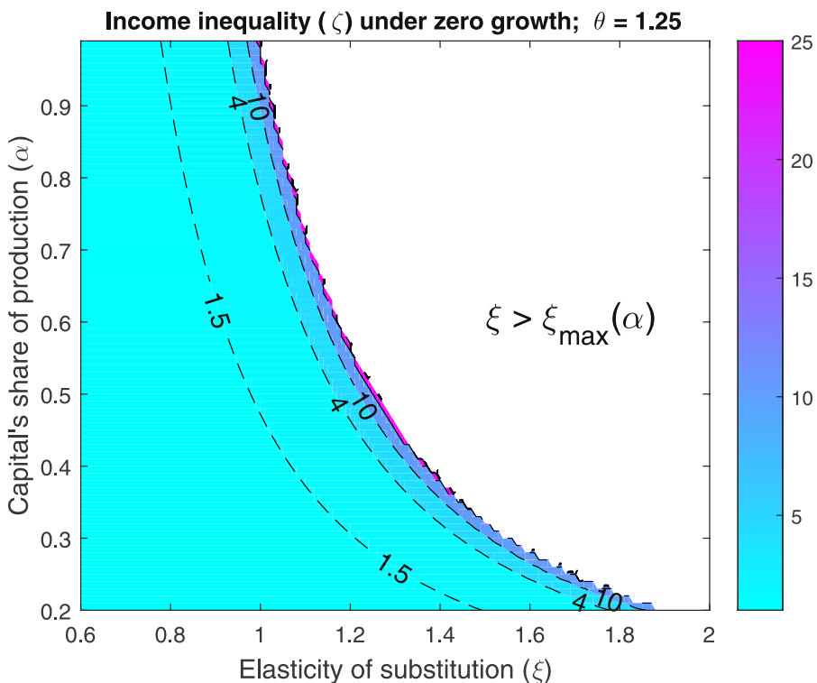
Fig. 7. Income inequality in a zero growth steady state.
