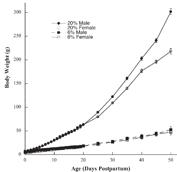
Fig. 1. Mean ( \pm S.E.M.) body weights for male (solid symbols) and female (open symbols) rats raised on a 20% protein diet (circles) and rats raised on a 6% protein diet (squares) from birth (0 days) to 50 days postnatal. Mean body weights for rats fed the 6% protein diet were significantly less than rats fed the 20% protein diet beginning at birth and extending through P50.
