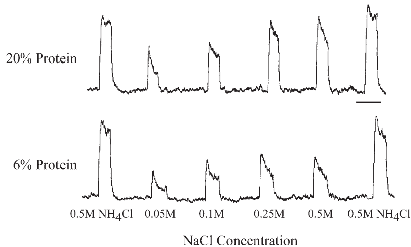
Fig. 2. Integrated responses from the chorda tympani nerve to a concentration series of NaCl and to 0.5 M \text{NH}_4\text{Cl} in a rat raised on a 20% protein diet (20% protein) and in a rat raised on a 6% protein diet (6% protein). Scale bar=1 min.
